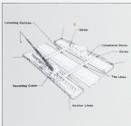
The Lay Barge. The tube is positioned for lowering between the catamaran barges of the lay barge. Additional concreting adds the proper weight for lowering the tube.
