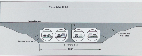
Cross section of the B-line tunnel
